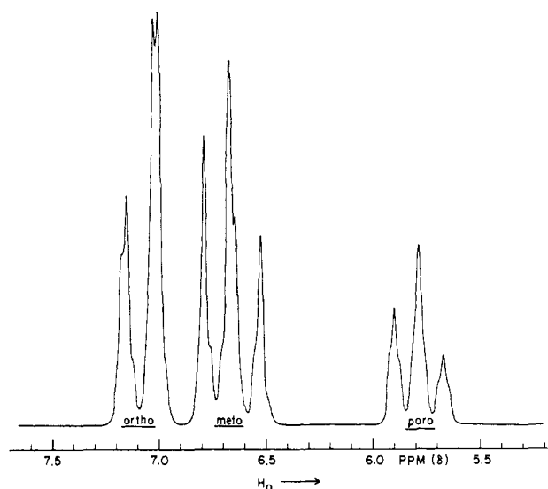
Figure 2. Calculated nmr spectrum for aromatic protons in diphenylcyclopropylcarbinylpotassium (XIV), using \nu_0 = 7.06 ppm.
